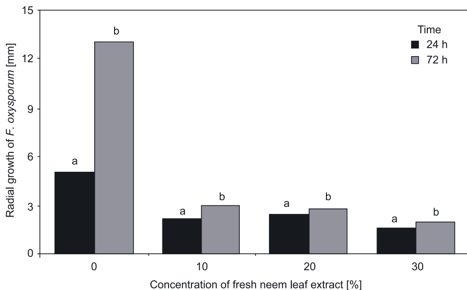
Fig. 1. Effect of fresh neem leaf extract on the growth of F. oxysporum on PDAS in 8.5 cm diameter agar plate at 24 and 72 hours. For each time period, bars bearing the same letter are not statistically significant at 5% probability
