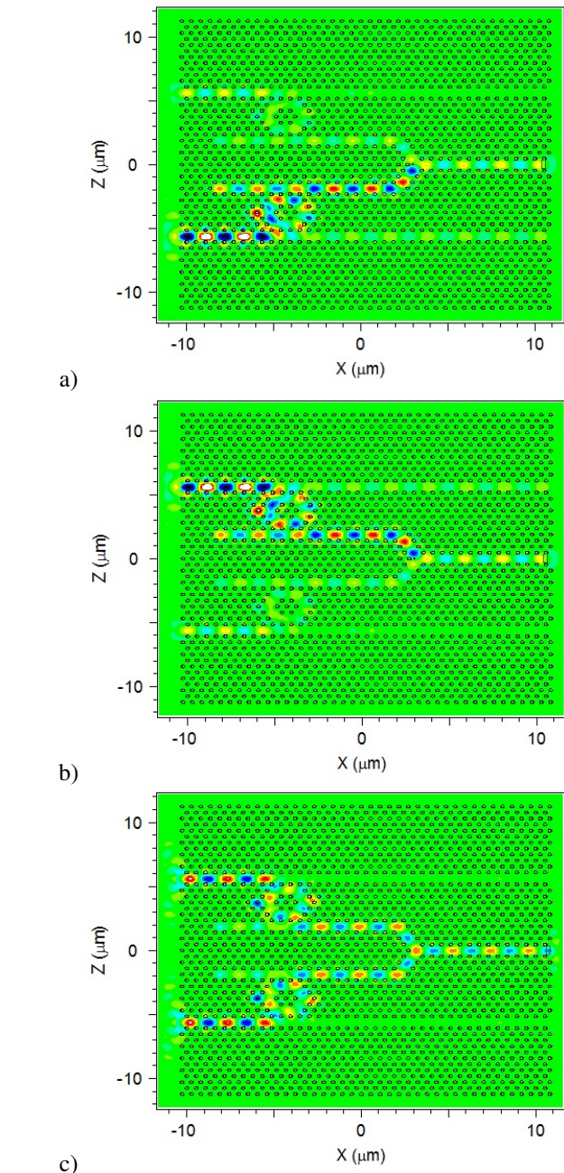
Fig. 6. Power flow indicator diagram of all optical OR gate
