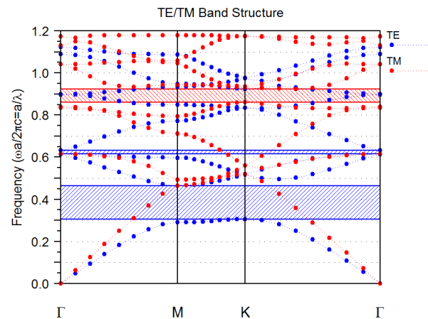
Fig. 1. PBG of proposed 2-D PhCs lattice structure
