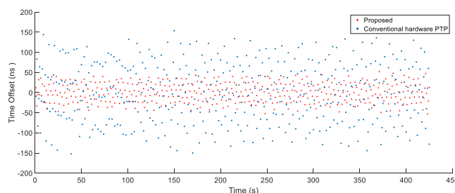
Fig. 11. Comparison of hardware timestamping and optimized algorithm
