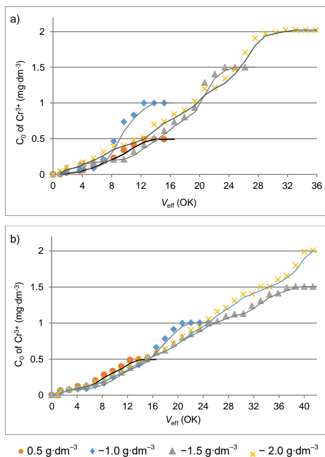
Fig. 1. Saturation curves of bentonite with a model solution with different concentration of Cr 3+ ( C_0 ):
