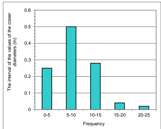
Fig. 4. Histogram of the karst crater distribution by diameter at the spot; source: own study
