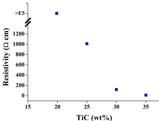
Fig. 9. Resistivity of the composite as a function of TiC
