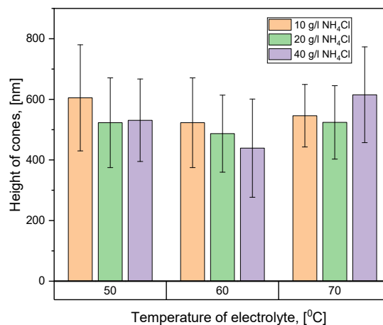
Fig. 4. The average values of cones height dependence on an amount of crystal modifier and electrolyte temperature
