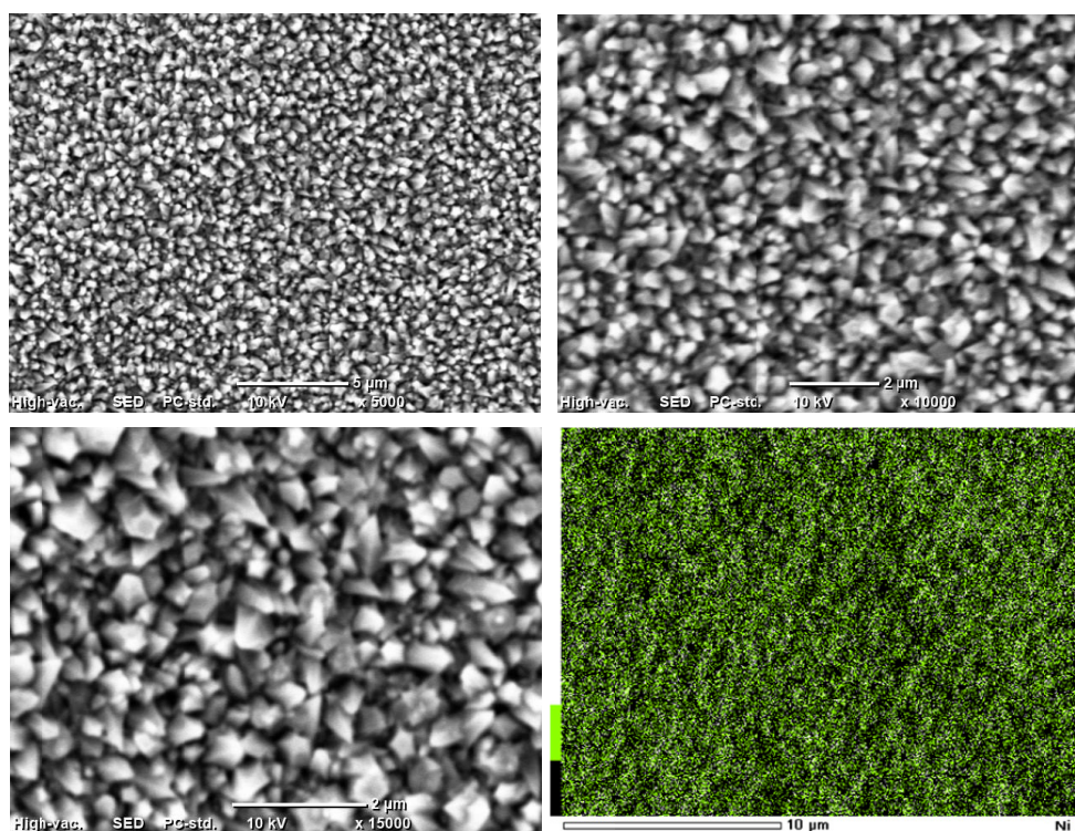
Fig. 2. SEM photos and mapping analysis of sample electrodeposited at 60^\circ\text{C} , i = 10 \text{ mA/cm}^2 with 20 \text{ g/l} \text{NH}_4\text{Cl}
