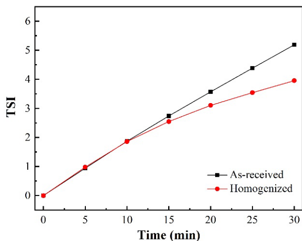
Fig. 2. TSI value of the Y_2O_3 suspension before and after homogenization
