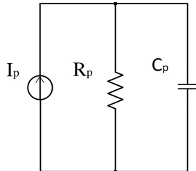
Fig. 7. Electrical equivalent model of a PZ Cantilever Plate
