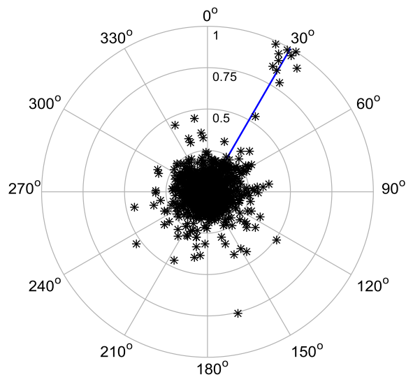
Fig. 26. Azimuth measurement results; SNR_i = -13 dB (parameters as in Fig. 24).
