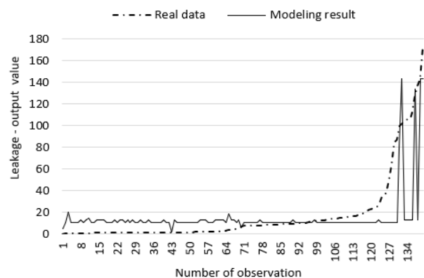
Fig. 5. Fifth set modelling results, in the basic criterion, with 2 hidden neurons and 20% values in the test set
