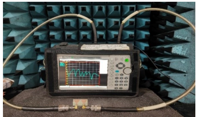
Fig. 8. Measurement setup of the proposed Multi-band MIMO antenna
