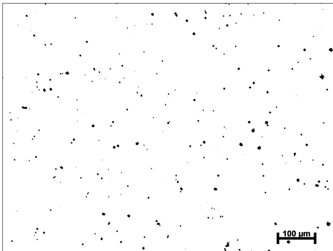
Fig. 1. The non-etched microstructure of Ti6Al4V
