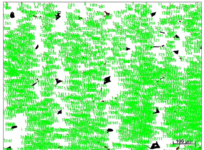
Fig. 4. Software image of CoCrW specimens prepared by AM technology
