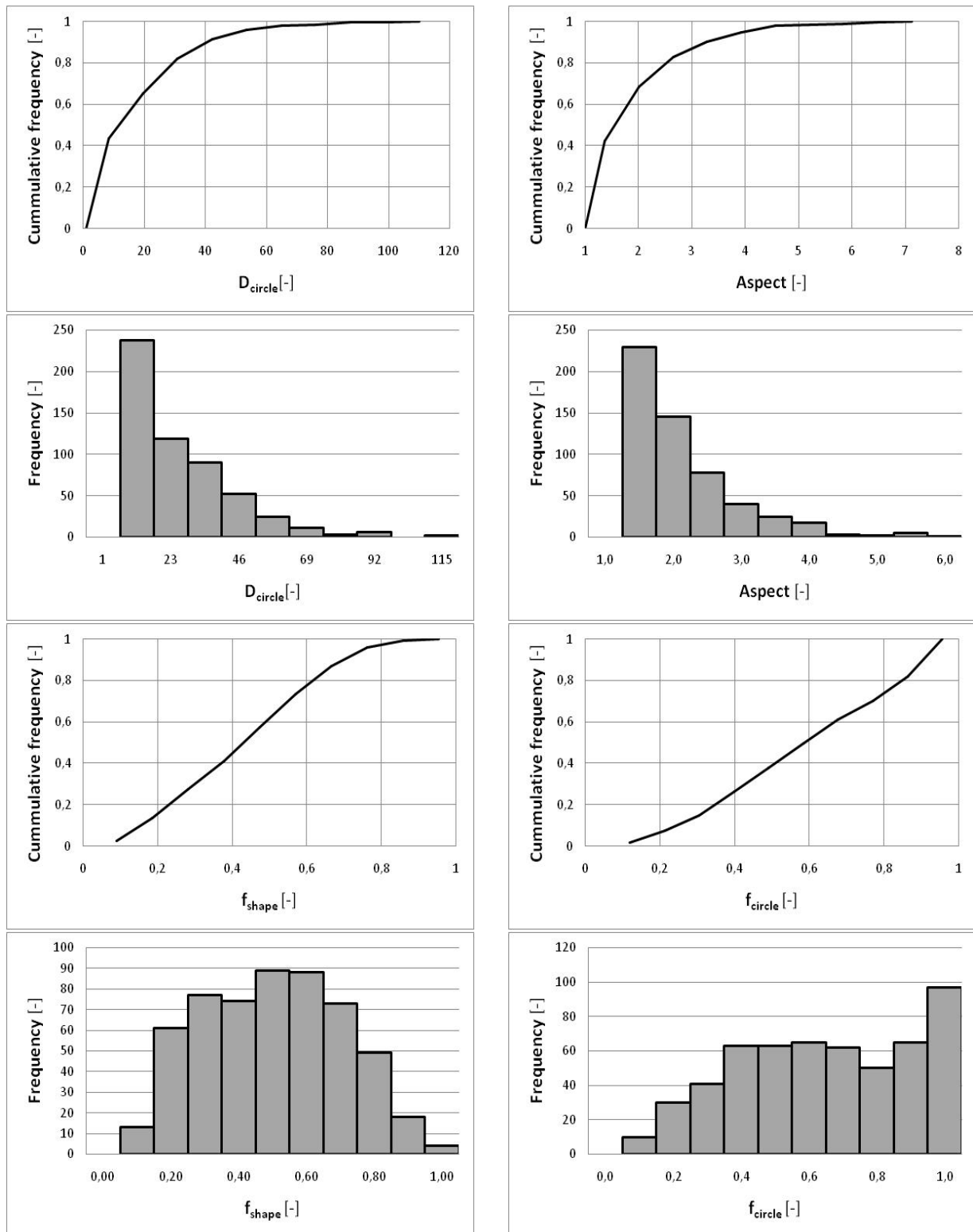
Fig. 6. The distribution histograms and the cumulative frequency of D_{circle} , Aspect, f_{shape} , and f_{circle} in CoCrW
