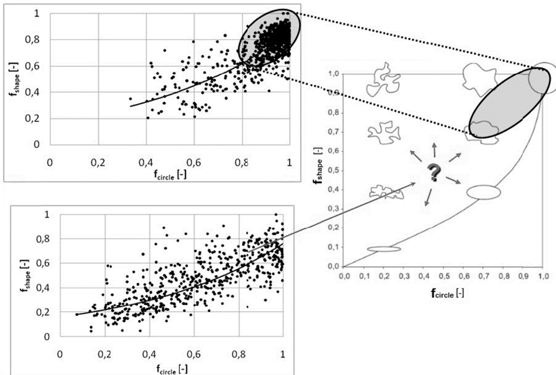
Fig. 7. The results f_{circle} and f_{shape} of both alloys
