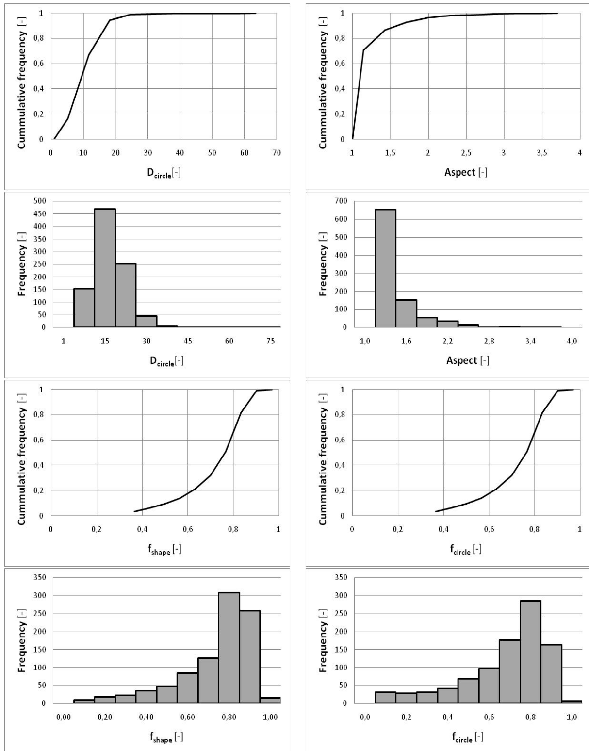
Fig. 5. The distribution histograms and the cumulative frequency of D_{circle} , Aspect, f_{shape} and f_{circle} in Ti6Al4V
