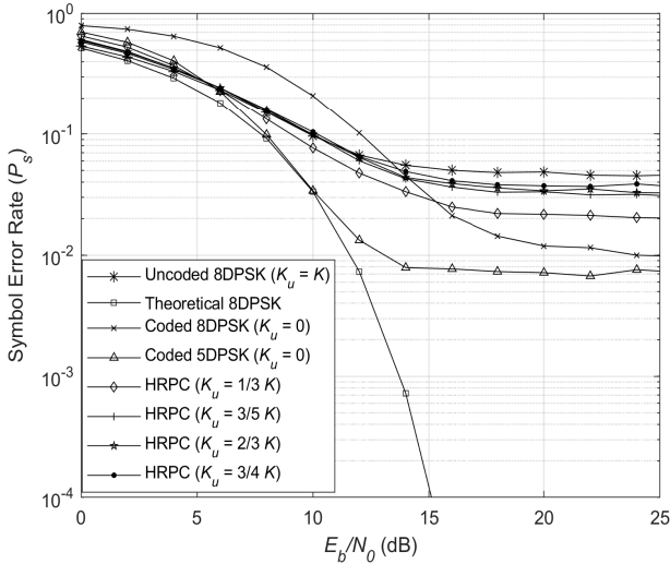
Fig. 7. Symbol error rate curves for modified DPSK modulator schemes under AWGN, frequency selective fading and impulsive noise channel.
