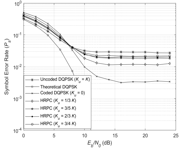
Fig. 5. Symbol error rate curves for DQPSK schemes under AWGN, frequency selective fading and impulsive noise channel.
