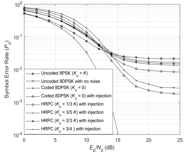
Fig. 9. Symbol error rate curves for injection coding schemes under AWGN and frequency selective fading channel.
