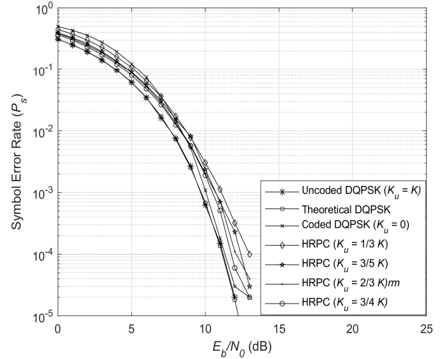
Fig. 3. Symbol error rate curves for DQPSK schemes under AWGN.
