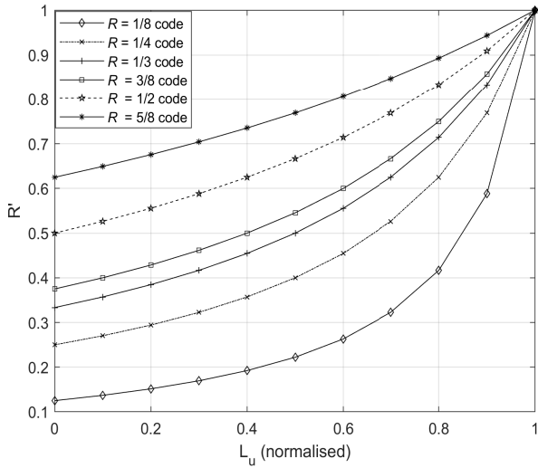
Fig. 2. Effective rates of codes with different R for various K_u s.
