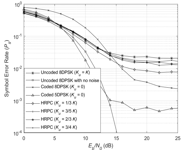
Fig. 6. Symbol error rate curves for modified DPSK modulator schemes under AWGN and frequency selective fading channel.
