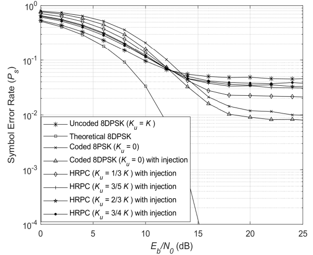
Fig. 8. Symbol error rate curves for injection coding schemes under AWGN, frequency selective fading and impulsive noise channel.
