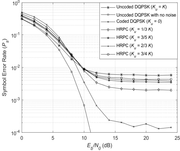
Fig. 4. Symbol error rate curves for DQPSK schemes under AWGN and frequency selective fading channel.
