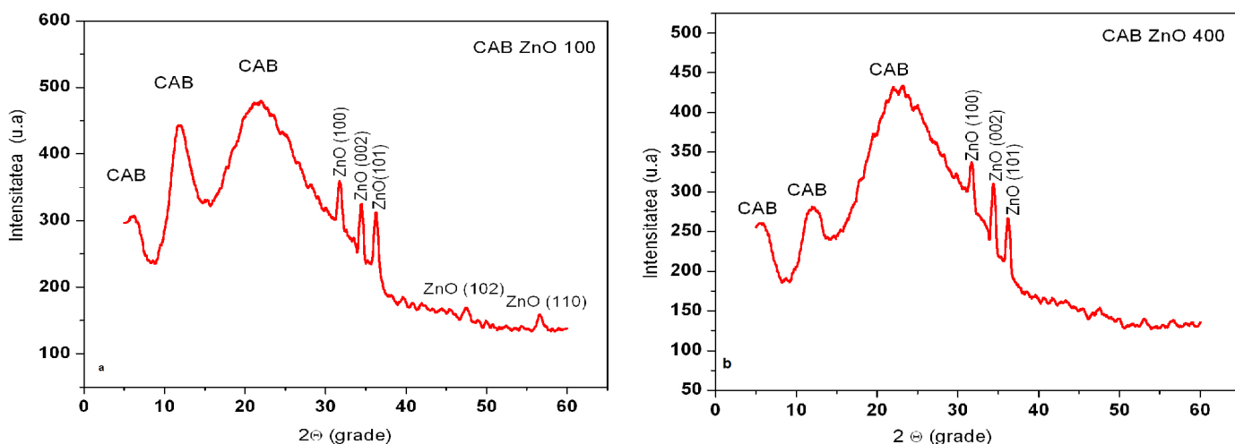
Fig. 3. X-ray diffractograms ( \text{CuK}\alpha ) recorded for composite nanofibers: a) CAB ZnO 100, b) CAB ZnO 400
