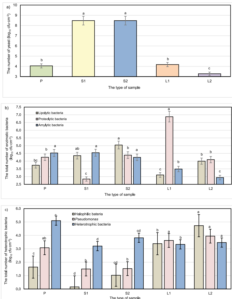
Fig. 2. Total counts recorded of microorganisms in port waters and balast water samples from ships operating in European and ocean waters: a) yeasts, b) enzymatic bacteria (lipolytic, proteolytic, amylytic), c) halophilic bacteria, Pseudomonas , heterotrophic bacteria; a, b, c, d, ab, bc, cd = statistical significance of individual groups of microorganisms between samples; source: own study
