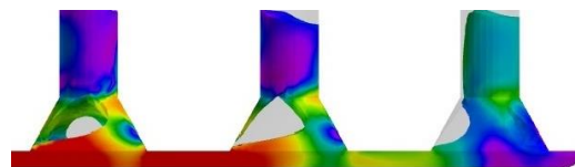
Fig. 3. Melt velocity in the construction without filter
