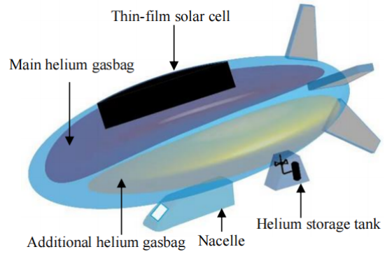
Fig. 1. Structure model of manned airship
