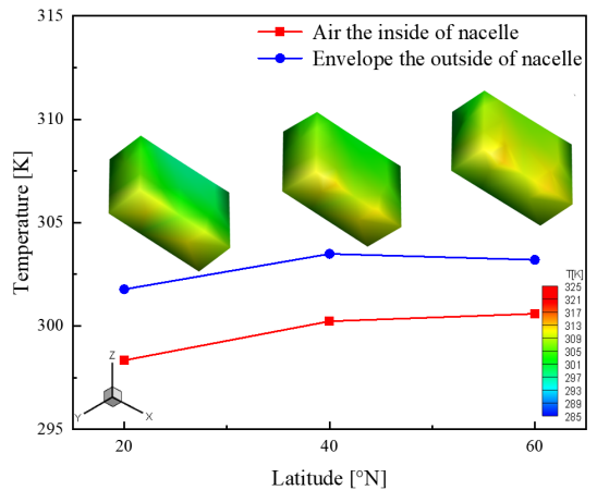
Fig. 15. Temperature variation of the airship nacelle at different latitudes
