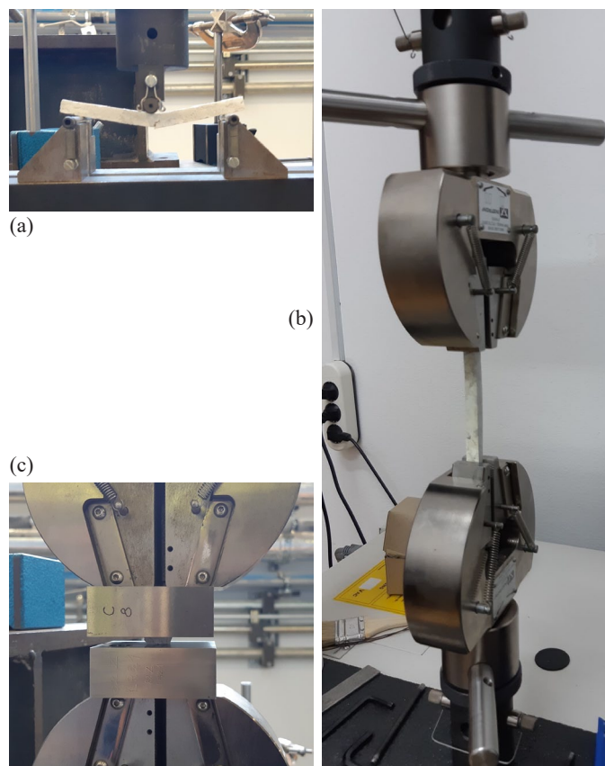
Fig. 4. Testing equipment for: (a) flexural test; (b) tensile test; (c) compression test
