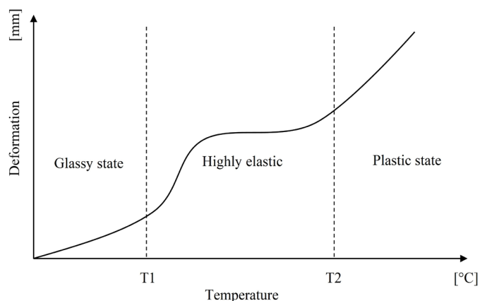
Fig. 2. Deformation versus temperature of a thermoplastic material [33]
