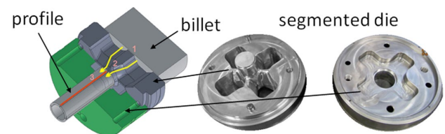
Fig. 1. An example of die design for a regular tube profile extrusion (Extral), includes scheme of the extrusion process and segmented die before assembly
