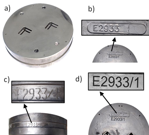
Fig. 3. Identification of the die tool using various techniques: a) view of a typical die for the aluminum extrusion, b) pressing method, c) engraving technique, d) laser marking method
