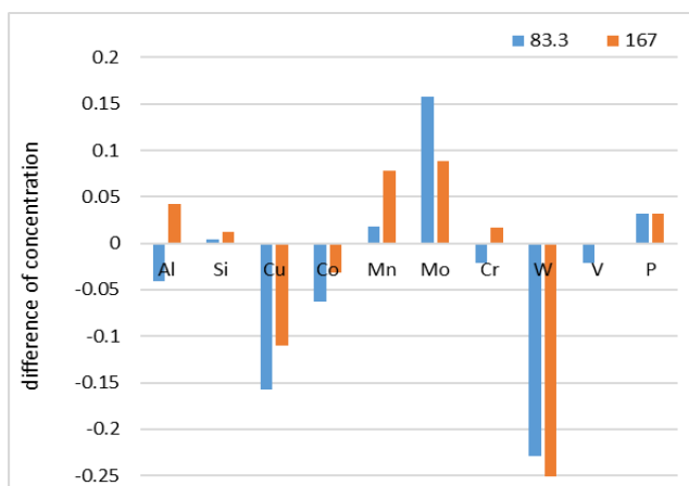
Fig. 8. Difference of concentration elements between cementite and pearlite, v = 83.3 and 167 \mu\text{m/s}
