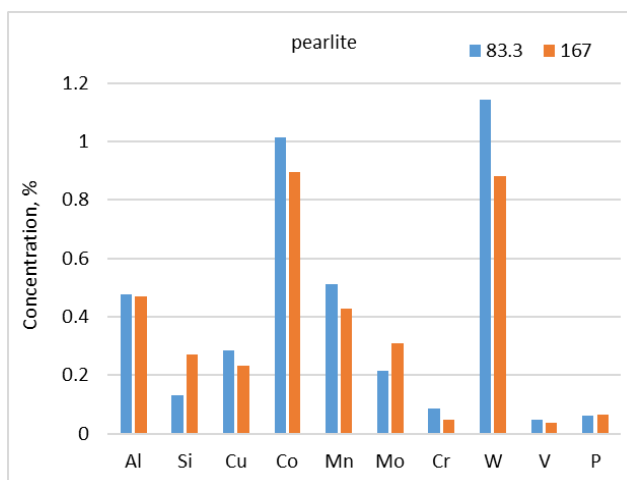
Fig. 7. Concentration of elements in ledeburitic pearlite, v = 83.3 and 167 \mu\text{m/s}
