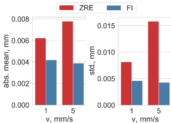
Fig. 12. Comparison of the abs. mean and standard deviation of the 3D deviations of the data measured with the use of different scanning speeds ( res=0.2 mm) and determined by using the Zeiss Reverse Engineering and Focus Inspection software
