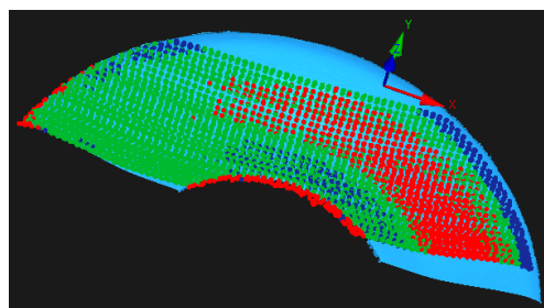
Fig. 6. View of the deviations in the ZRE software for the data measured by using the following parameters: v=1 mm/s, res=0.2 mm
