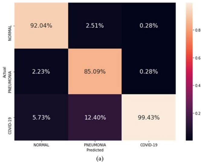
Fig. 10. The Confusion Matrix of: (a) The proposed model. (b) VGG-16. (C) Alex Net. (D) ResNet50
