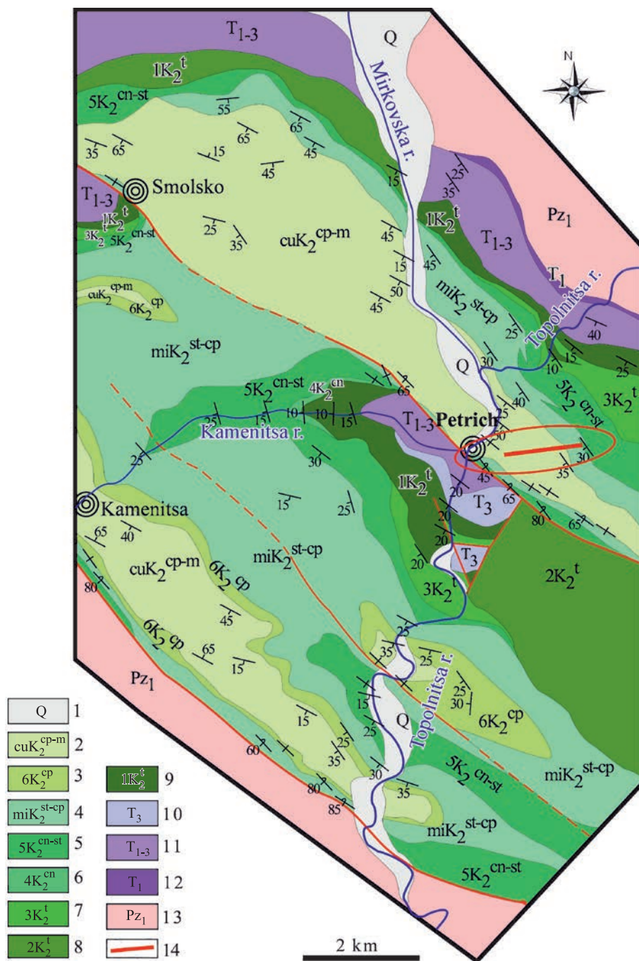
Text-fig. 2. Geological sketch map of the area of the Petrich village (after Vangelov et al. 2019). 1 – Quaternary (Q), 2 – Chugovitsa Formation (cuK 2 cp-m ), 3 – upper epiclastic unit (6K 2 cp ), 4 – Mirkovo Formation (miK 2 st-cp ), 5 – lower epiclastic unit (5K 2 cn-st ), 6 – marl-limestone unit (4K 2 cn ), 7 – volcanoclastic unit (3K 2 t ), 8 – Vran Kamak magmatic centre (2K 2 t ), 9 – basal terrigenous unit (1K 2 t ), 10 – Moesian Terrigenous-Carbonate Group (T 3 ), 11 – Iskar Carbonate Group (T 1-3 ), 12 – Petrohan Terrigenous Group (T 1 ), 13 – Palaeozoic high-grade metamorphites (Pz 1 ), 14 – location of the section studied.
