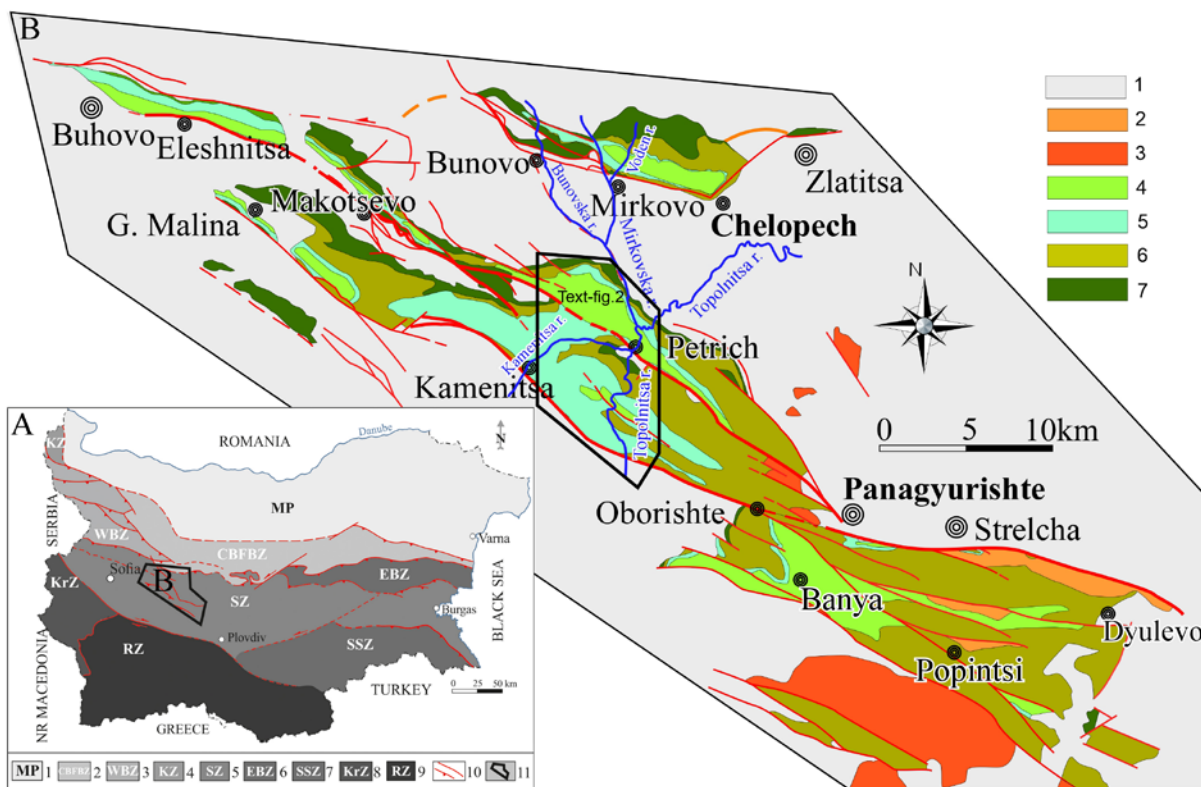
Text-fig. 1. Location of the study area. A – Tectonic sketch map of Bulgaria showing the position of the Chelopech and Panagyurishte strips (after Ivanov 2017): 1 – Moesian Platform, 2 – Central Balkan–Fore-Balkan Zone, 3 – West Balkan Zone, 4 – Kula Zone, 5 – Srednogorie Zone, 6 – East Balkan Zone, 7 – Sakar-Strandzha Zone, 8 – Kraisthe Zone, 9 – Rhodope Zone, 10 – Main faults and thrusts, 11 – outline of the study area. B – Geological sketch map of the Upper Cretaceous volcano-sedimentary sequences exposed in the Chelopech and Panagyurishte strips (after Vangelov et al. 2019): 1 – pre-Cretaceous basement, 2 – Paleocene, 3 – Upper Cretaceous plutons, 4 – Chugovitsa Formation, 5 – Mirkovo Formation, 6 – volcano-terrigeneous complex, 7 – basal terrigenous unit.
