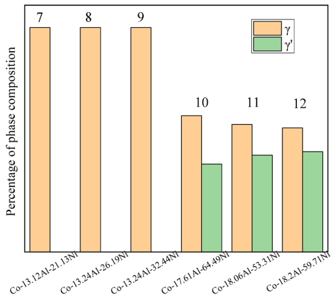
Fig. 5. Calculated phase content of the referred EDS test points in sublayers B and C used JMatpro
