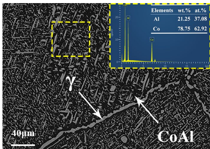
Fig. 2. SEM morphology of Co40Al master alloy
