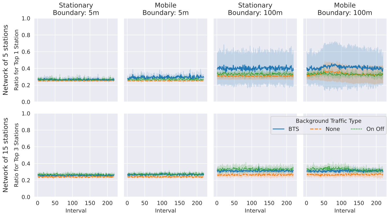
Fig. 7. The ratio of aggregated throughput of top N stations to total network throughput over time. Stations' mobility, type of background traffic, network size, and station location restriction are parameterised. The translucent bands represent the standard deviation of the collected data.
