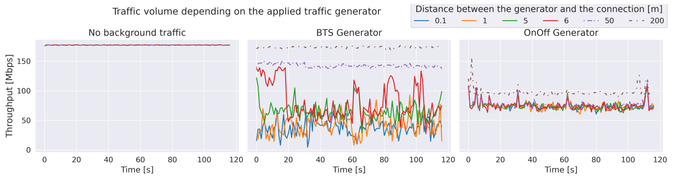
Fig. 3. Connection throughput depending on the background traffic generator used.
