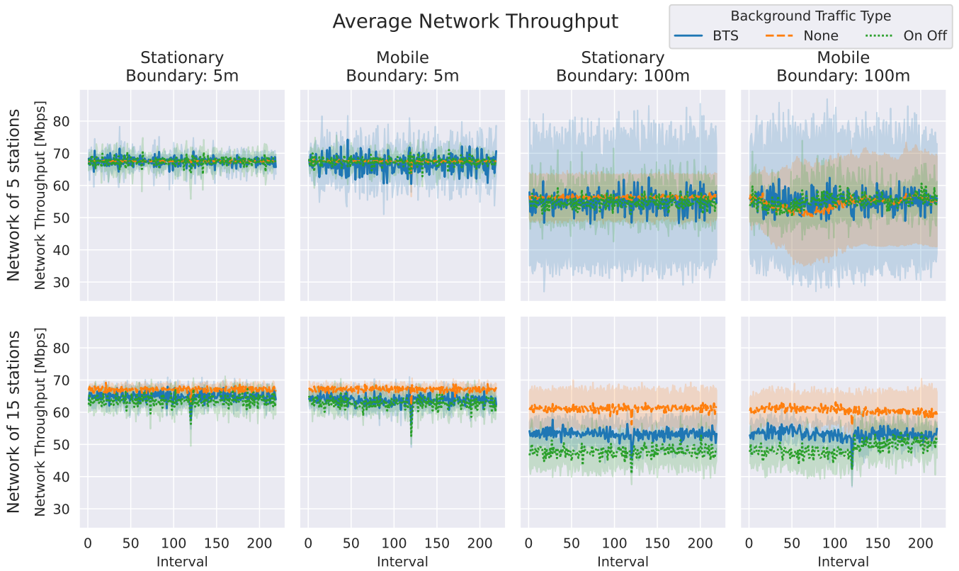
Fig. 6. Average network throughput under various configurations. Stations' mobility, type of background traffic, network size, and station location restriction are parameterised. The translucent bands represent the standard deviation of the collected data.
