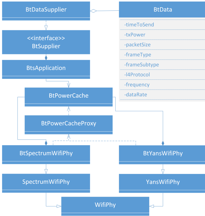
Fig. 1. UML diagram of main modules of BTS extension for ns-3 simulator.
