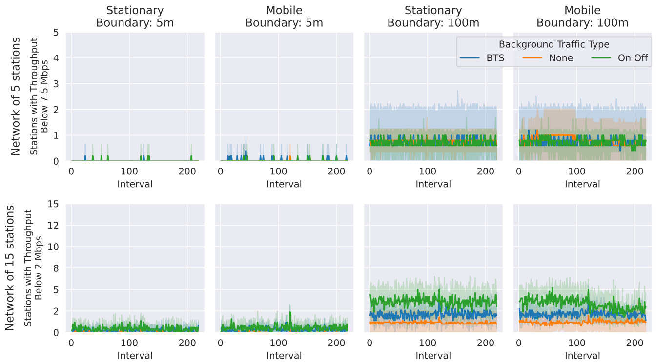
Fig. 8. Number of stations with throughput below the threshold over time. Stations' mobility, type of background traffic, network size, and station location restriction are parameterised. The translucent bands represent the standard deviation of the collected data.
