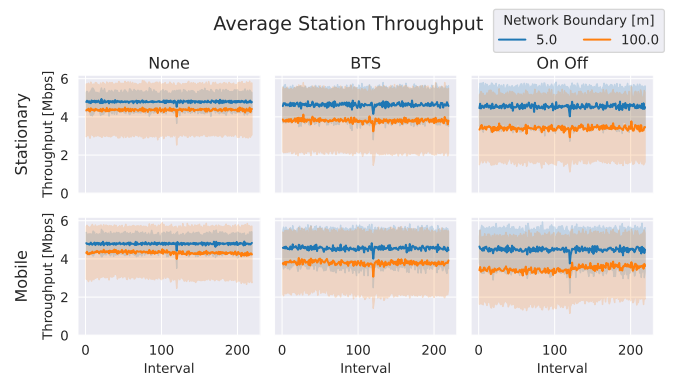
Fig. 5. Average station throughput in the 15 node network under various configurations. Stations' mobility, type of background traffic, and station location restriction are parameterised. The translucent bands represent the standard deviation of the collected data.
