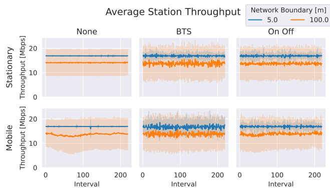
Fig. 4. Average station throughput in the 5 node network under various configurations. Stations' mobility, type of background traffic, and station location restriction are parameterised. The translucent bands represent the standard deviation of the collected data.
