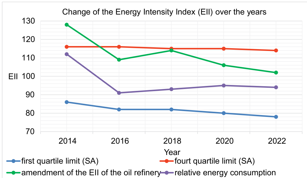
Fig. 2. Change in the EII energy index and relative energy consumption
