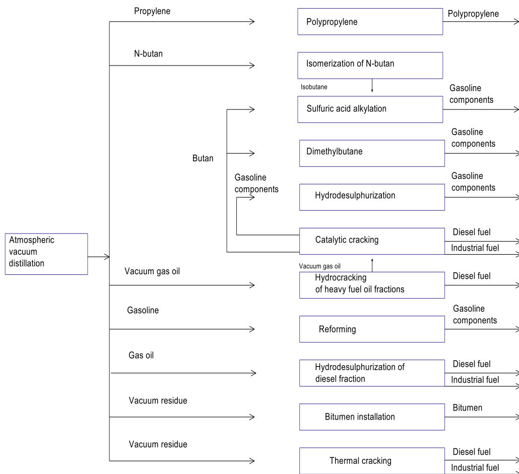
Fig. 1. Block diagram of the refinery
