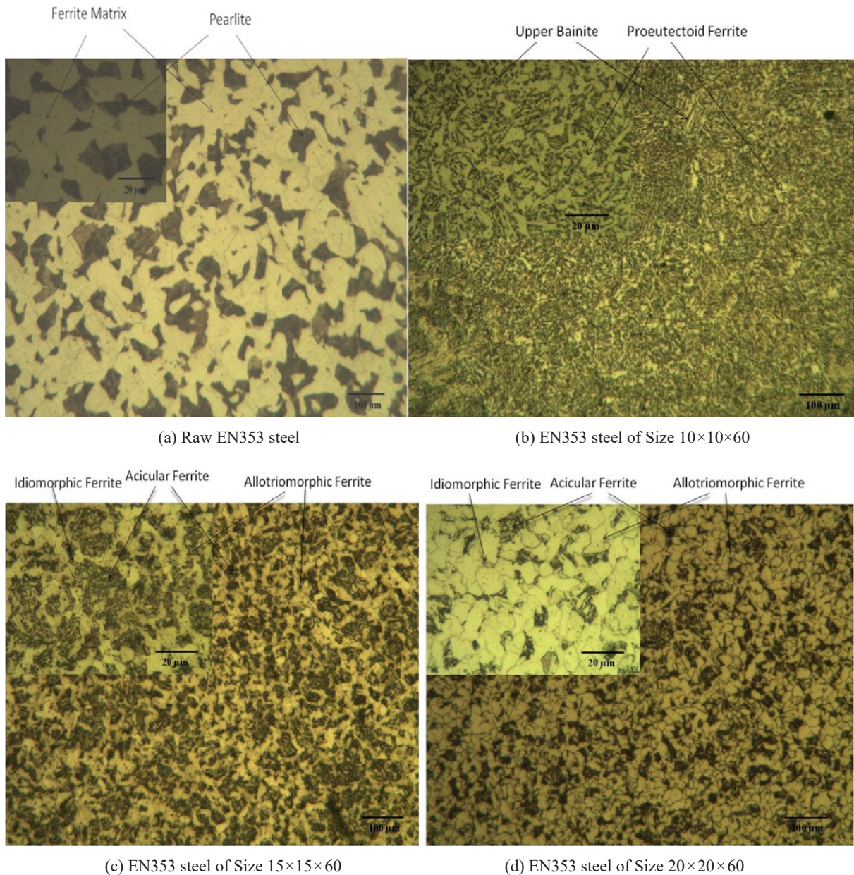
Fig. 6. Microstructural analysis of different sized EN353 specimens at 100x & 400x magnification
