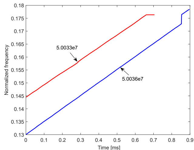
Fig. 15. Instantaneous frequency extraction of target highlights.
