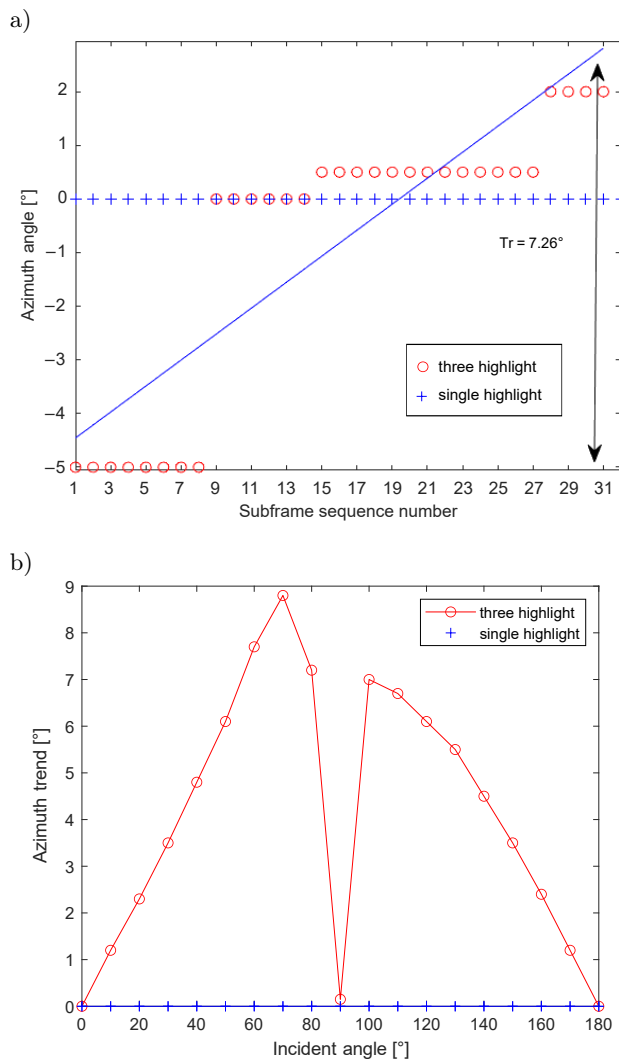
Fig. 4. Echo azimuth trend estimation: a) azimuth trend of 60^\circ incident angle; b) azimuth trend of different incident angles.
