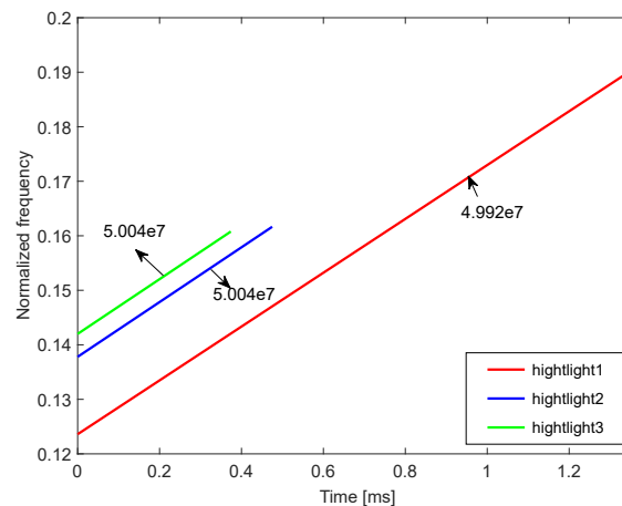
Fig. 20. Instantaneous frequency extraction of target highlights.
