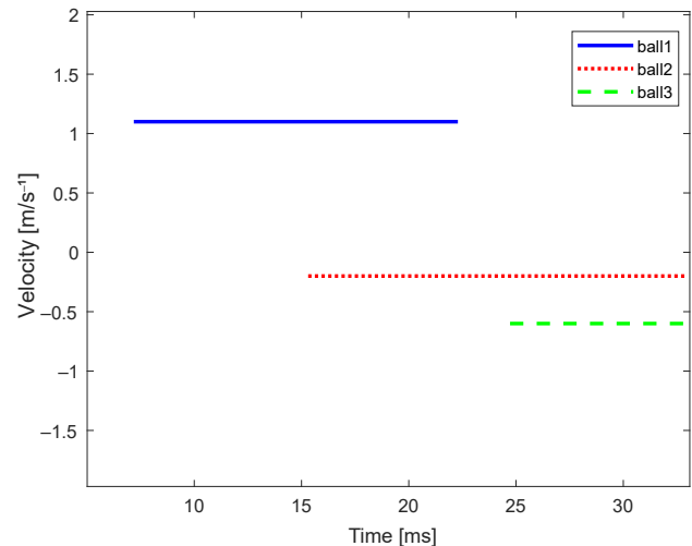
Fig. 7. Speed estimation.
