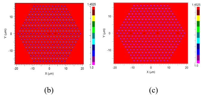
Fig. 3. The cross-section of the 1*4 wavelength demux: (a) XZ plane at y = 0 mm. (b) XYPlane at z = 0 mm. (c) XY plane at z = 6\text{mm}
