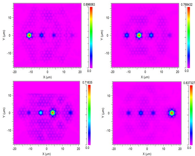
Fig. 5. XY cross-section optical signals simulations intensity demultiplexing 1*4 (a: \lambda=0.85\mu\text{m} ; b: \lambda=1.1\mu\text{m} ; c: \lambda=1.19\mu\text{m} ; d: \lambda=1.35\mu\text{m} ) at z=6\text{mm}
