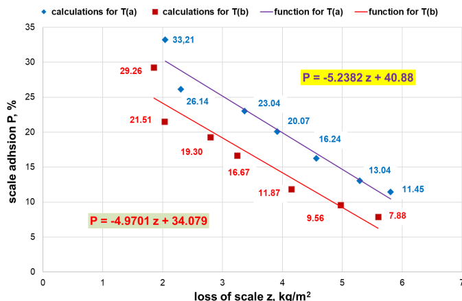
Fig. 4. Dependence of scale adhesion on steel loss
