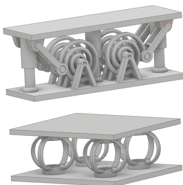
Fig. 1. Developed models of anti-vibration systems with external dimensions: model I – 24 × 77 × 29.6 mm (top); model II – 60 × 60 × 25.3 mm (bottom).
