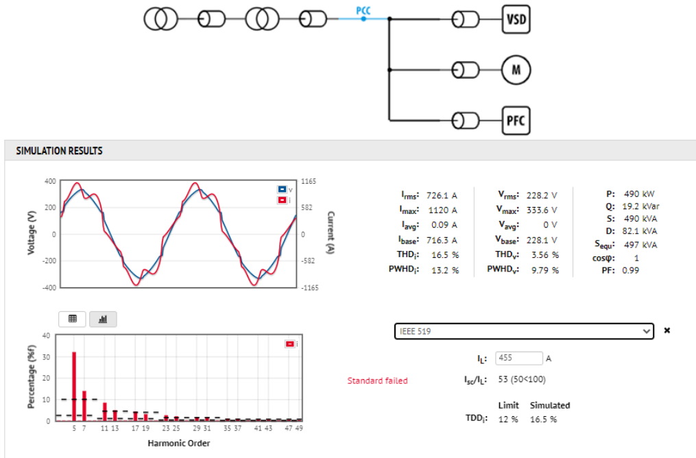
Fig. 8. Scenario 2 (with reactive power compensation device 200 kVar, 189 Hz)
