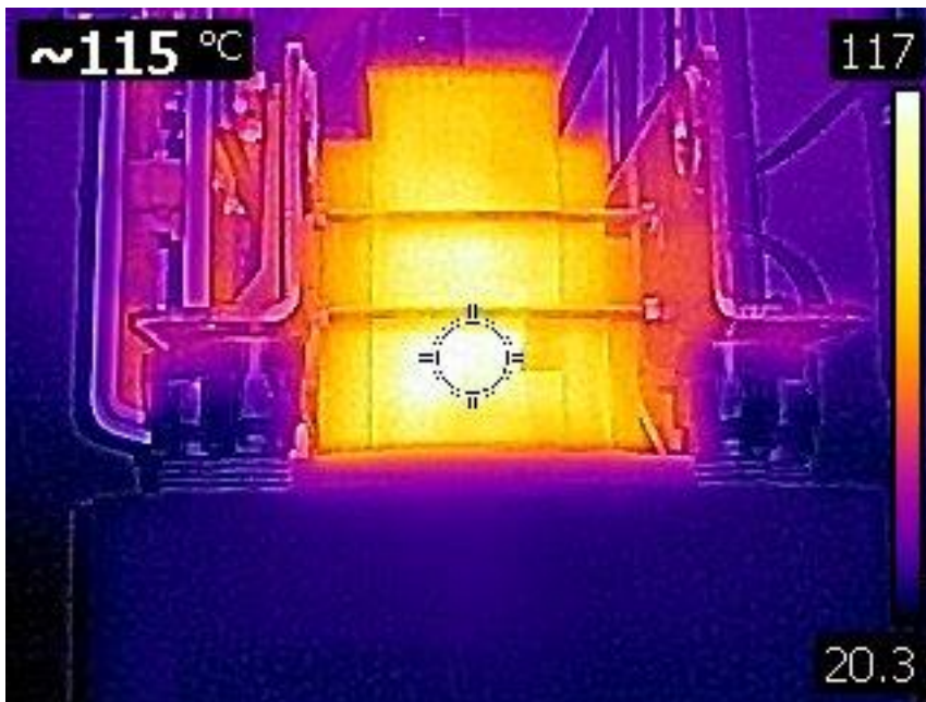
Fig. 15. Heating of the dry transformer magnetic circuit under the influence of harmonic distortion
