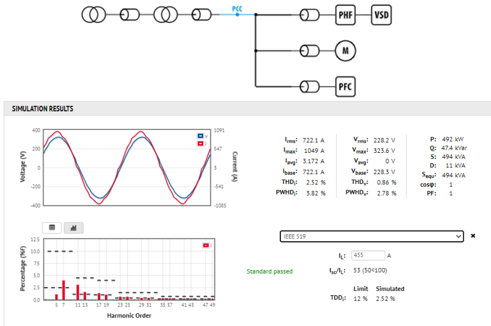
Fig. 10. Scenario 4 (with additional passive filter)
