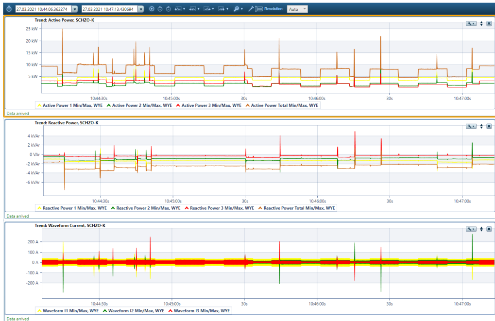
Fig. 5. Graphs of measurement of active, reactive power, and current waveform on the LED floodlight power line
