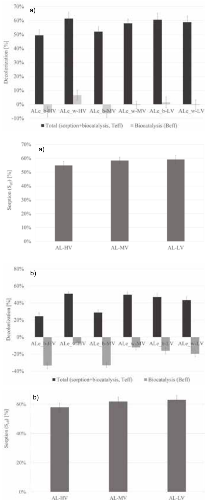
Figure 5. Decolorization of a) IC in a mixture and b) MB in a mixture
