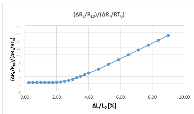
Fig. 11. Quotient of relative changes of longitudinal and transversal resistance during stretch tests.
