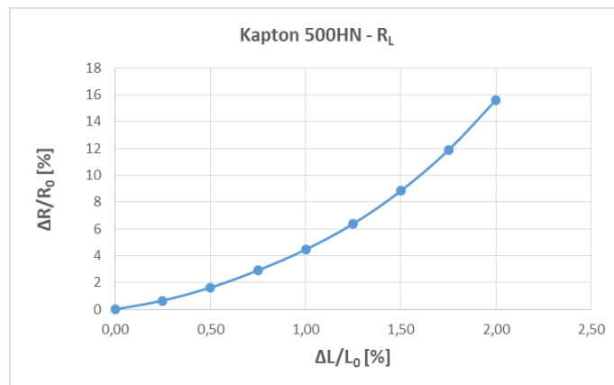
Fig. 10. Relative changes of electrical resistance during stretch tests in applicable strain range
