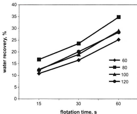
Fig. 3. Water recovery in the froth product as a function of the flotation time for the pulp densities of 60, 80, 100 and 120 \text{g/dm}^3
