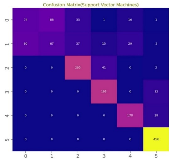
Fig. 6. Confusion matrix of SVM
