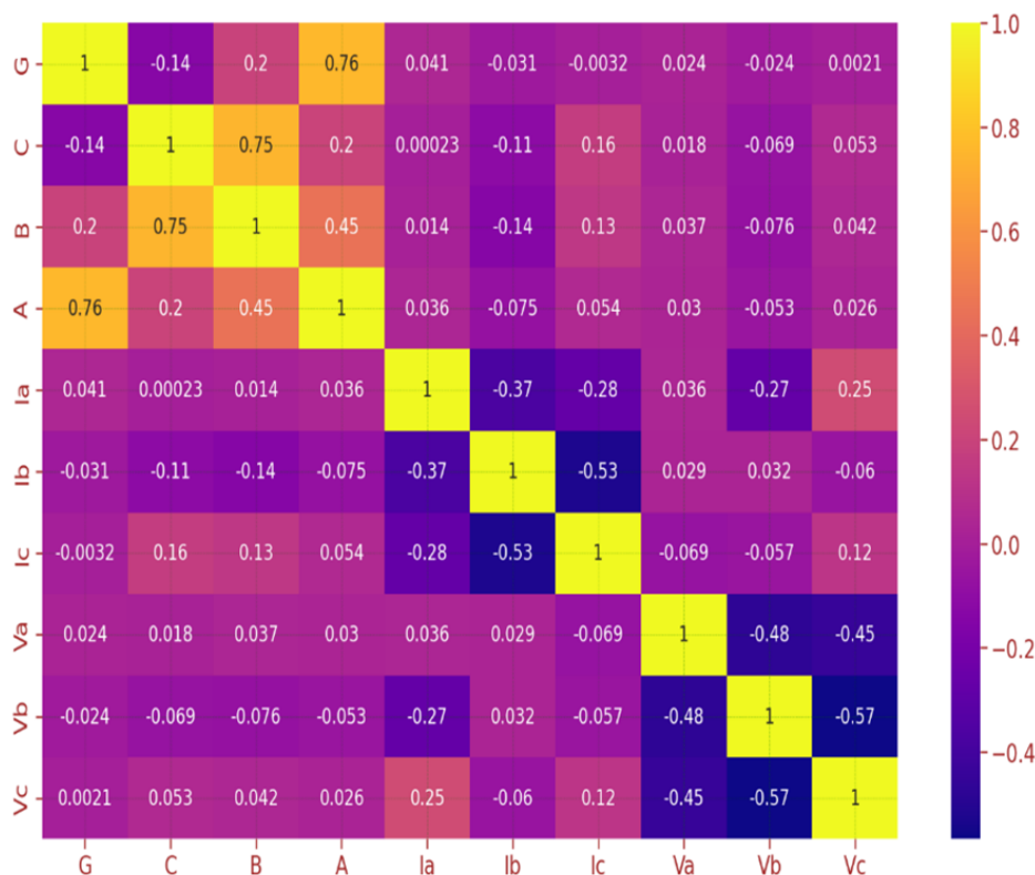
Fig. 3. Correlation matrix
