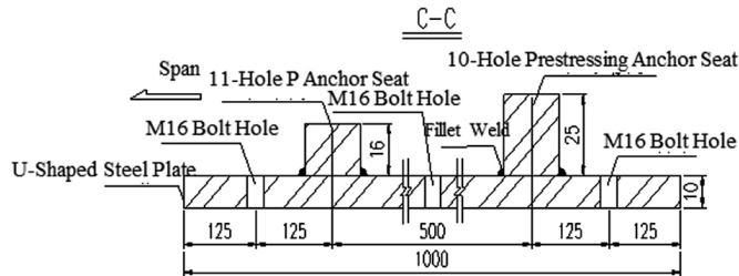
Fig. 8. Side elevation view of anchor 1 on the bottom of the beam (unite: cm)
