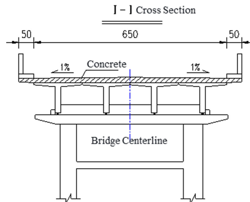
Fig. 2. Bridge cross-section drawing (unite: cm)
