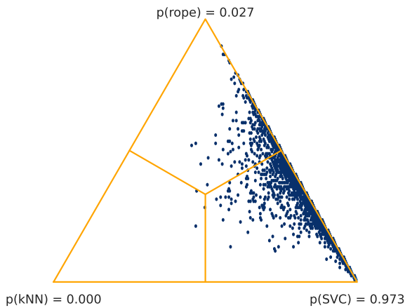
Fig. 4. Advantage of SVM over kNN in classification experiment for datasets with original labels and PQQ features, visualized using method from [42]. There is a 97.3% probability that average SVM performance is higher for a rope value of 2%.
