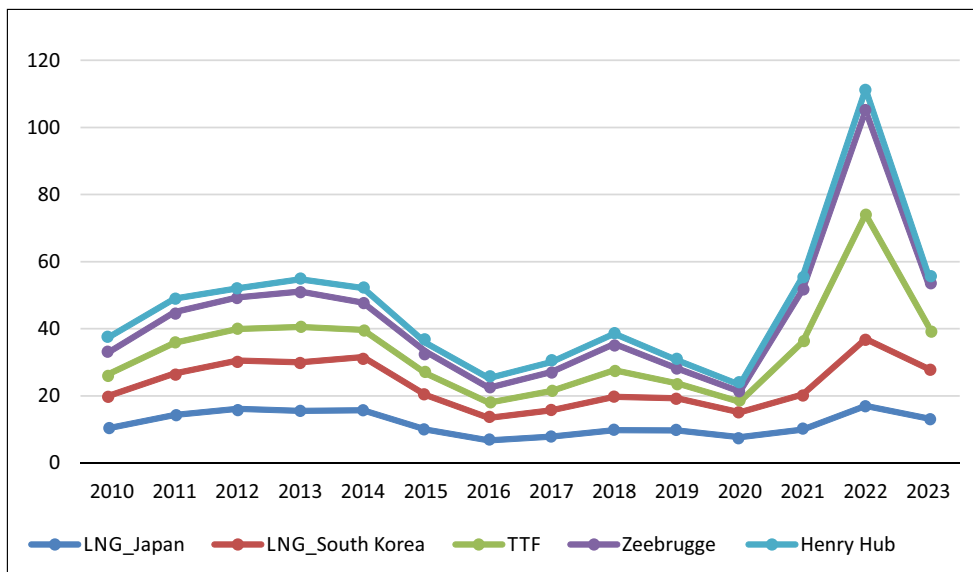
Fig. 5. Natural gas prices in 2010–2023 (US dollars per million BTU)
