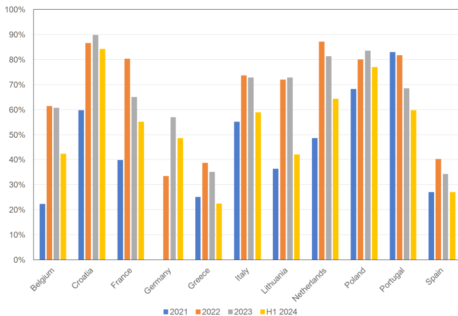
Fig. 14. Utilization of the available regasification capacity of LNG terminals in individual EU countries in 2021–2024. Source: GIE ALSI 2025
