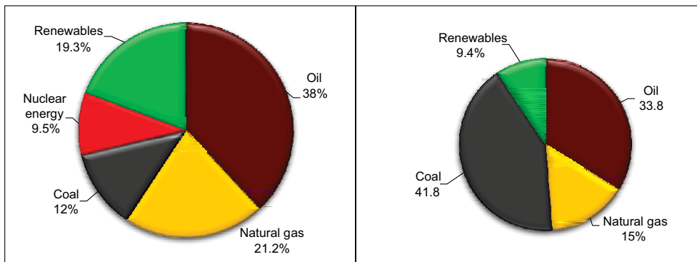
Fig. 2. Primary Energy: Consumption by fuel in Poland (right) and EU (left) – 2022 (%)
