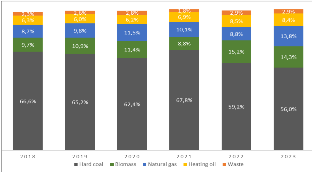
Fig. 4. Consumption of selected fuels for heat generation in cogeneration years 2018–2023 based on data published annually by the ERO
