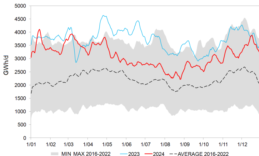
Fig. 10. Amount of gas regasified at LNG Terminals in the European Union in 2024 (compared to 2023 and to the range from 2016–2022), GWh/day Moving 7-day average.
