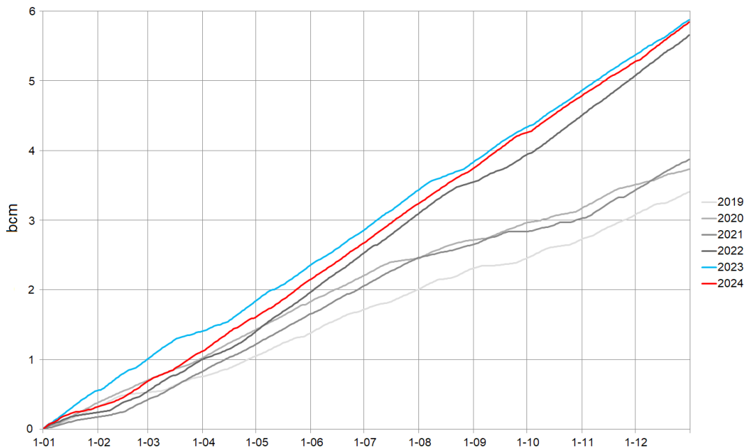
Fig. 12. Amount of natural gas regasified in Polish LNG Terminal in Świnoujście in 2019–2024 (cumulatively), bcm Source: ENTSG 2025
