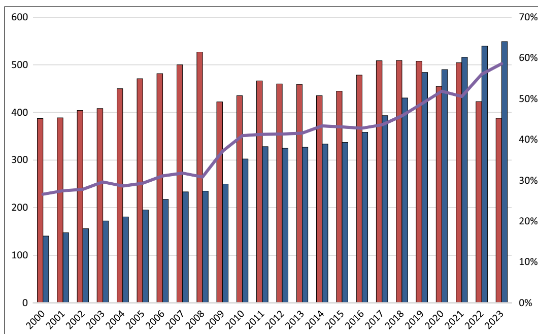
Fig. 1. Share of LNG in global natural gas trade in 2000–2023 (bcm – left axis; % – right axis)
