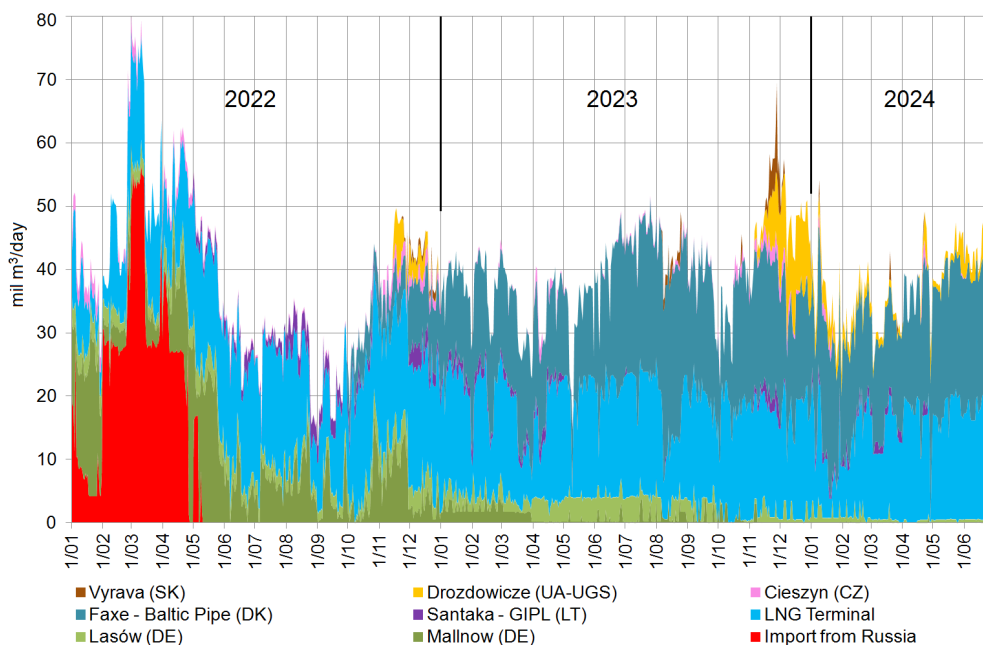
Fig. 9. Natural gas imports to Poland in 2022–2023 and in H1 2024 per day by entry points, million \text{m}^3/\text{day}
