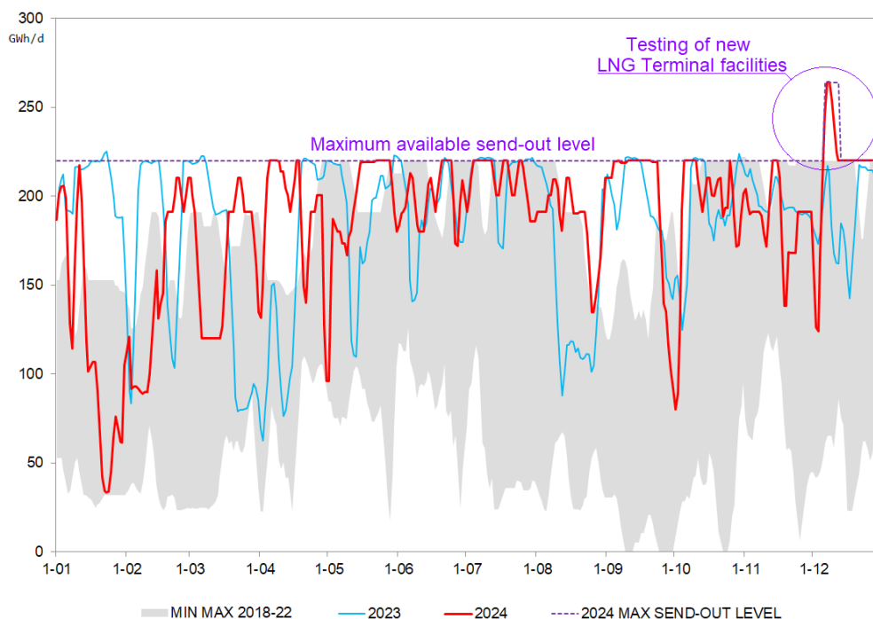
Fig. 15. Utilization of the regasification capacity of the LNG Terminal in Świnoujście in 2023 and 2024 compared to range from 2018–2022
