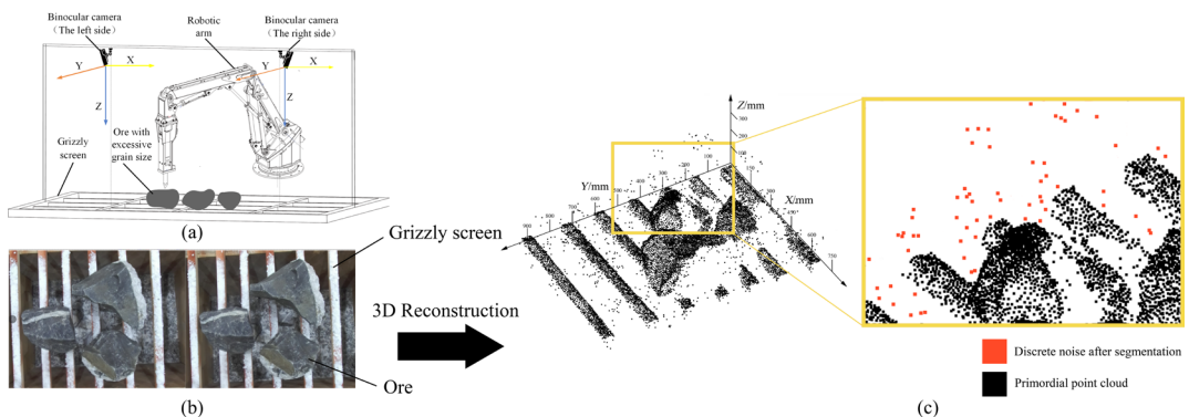
Fig. 1. 3D reconstruction of the ore on the grizzly screen (a) Binocular camera installation diagram, (b) Grizzly screen and ore captured by binocular camera, (c) Discrete noise in grizzly screen and ore point clouds
