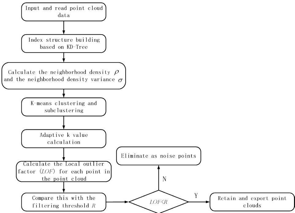
Fig. 2. K-neighborhood density filtering flowchart
