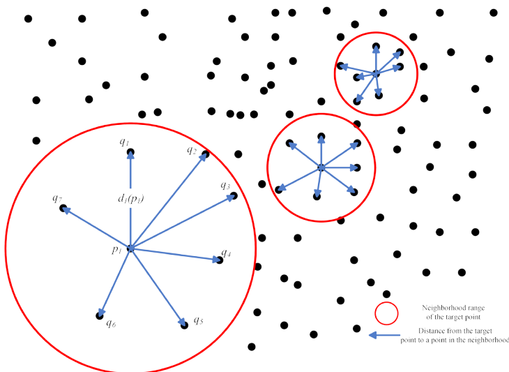
Fig. 3. Schematic of K-neighborhood density
