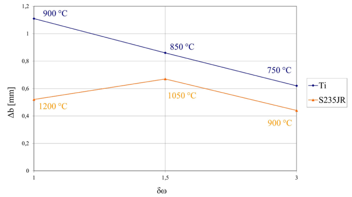
Fig. 5. Absolute expansion \Delta b as a function of the shape coefficient \delta\omega for samples rolled with a 10% reduction in a quarter arrangement with work rolls of 130 mm diameter
