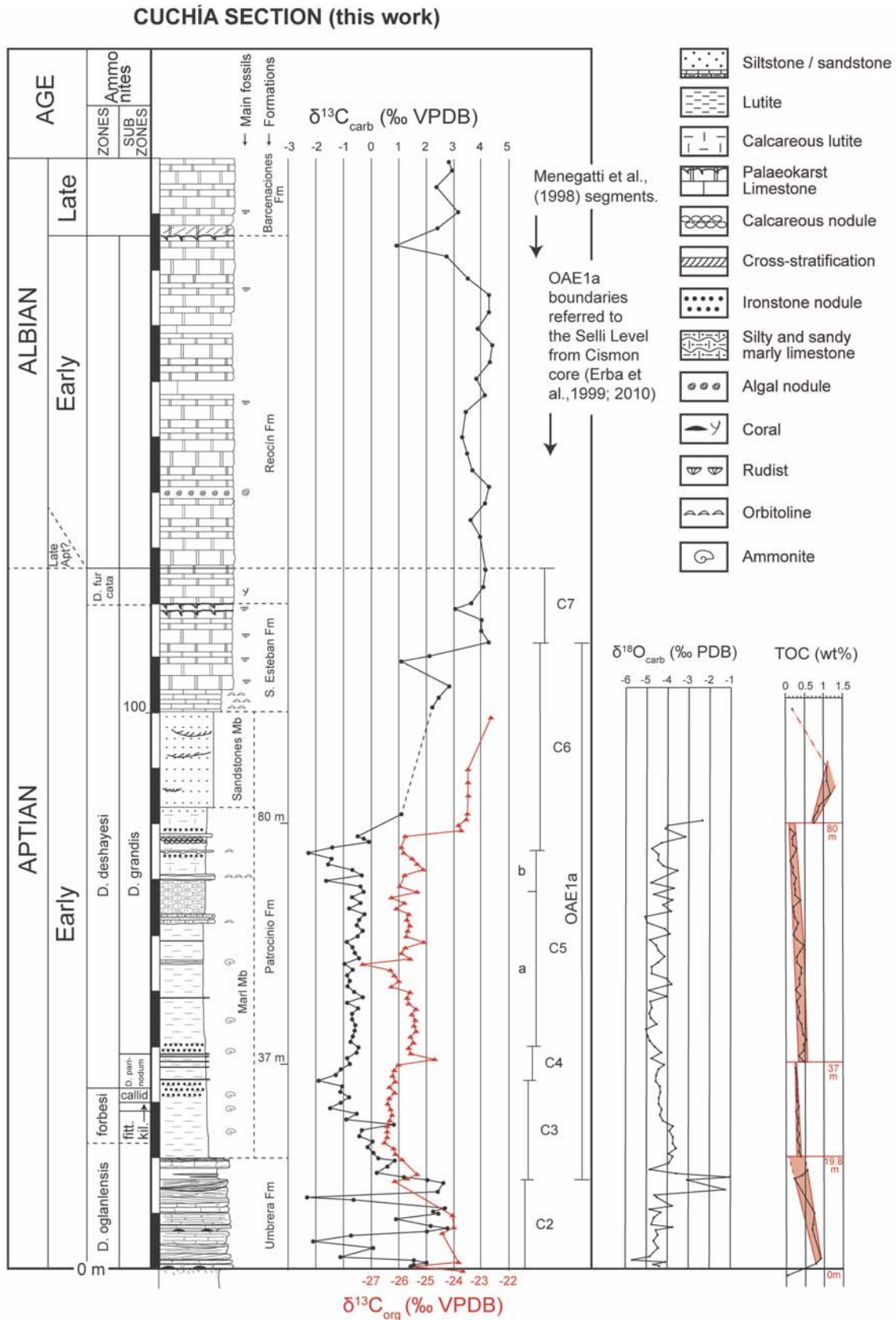
Text-fig. 2. Lithostratigraphy, age and geochemistry ( \delta^{13}C_{carb} , \delta^{13}C_{org} , \delta^{18}O_{carb} and TOC) of the Cuchía section
