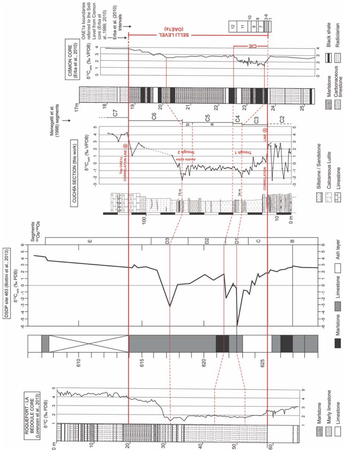
Text-fig. 4. Correlation of the \delta^{13}\text{C}_{\text{carb}} curve from Cuchía section with similar curves from Cismón core (Erba et al. 2010), Roquefort-La Bédoule core (Lorenzen et al. 2013) and DSDP site 463 (Bottini et al. 2013). All curves have been redrawn and enlarged. Correlation lines A (carbonate crisis level) and B (top of the OAE1a) link curve points with equivalent absolute values and shifts of the \delta^{13}\text{C}_{\text{carb}} trends, delimiting the Sellia Level and the negative carbon-isotope excursion (CIE). In Cuchía and DSDP 463 sections the Sellia-equivalent interval appears as a double negative trough in the curves. The second trough in Cuchía contains a double spike, as in the Roquefort-La Bédoule section. ^{187}\text{Os}/^{188}\text{Os} segments of Bottini et al. (2013) and CIE intervals of Erba et al. (2010) help to constrain the indirect correlation with Cuchía section
