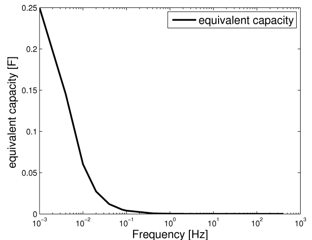
Fig. 11. Equivalent capacity C' of ultracapacitor 0.33F
