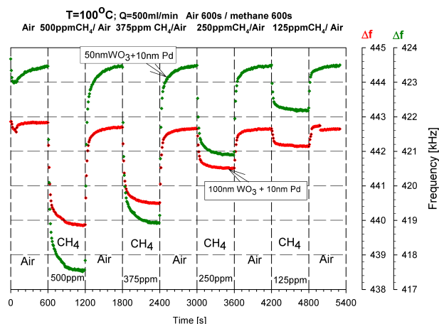
Fig. 11. Response of SAW sensor \Delta f with a WO_3 + Pd layer, 50 and 100 nm thick, to with concentrations of 500 to 125 ppm in air. Temperature of the sensor was 100^\circ C
