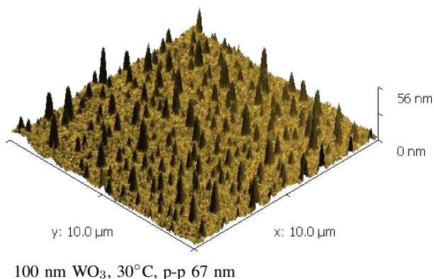
Fig. 9. Morphology of the surface of the WO_3 layer deposited on the substrate at a temperature of 30^\circ C
