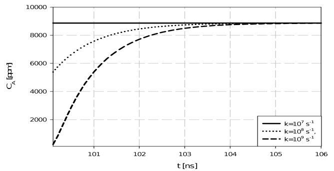
Fig. 5. The gas concentration profiles versus time at different rate constants k = 10^7 s ^{-1} , k = 10^8 s ^{-1} , k = 10^9 s ^{-1} and for C_{A,S} = 10000 ppm, n = 10 , D_K = 10^{12} nm ^2 s ^{-1}
