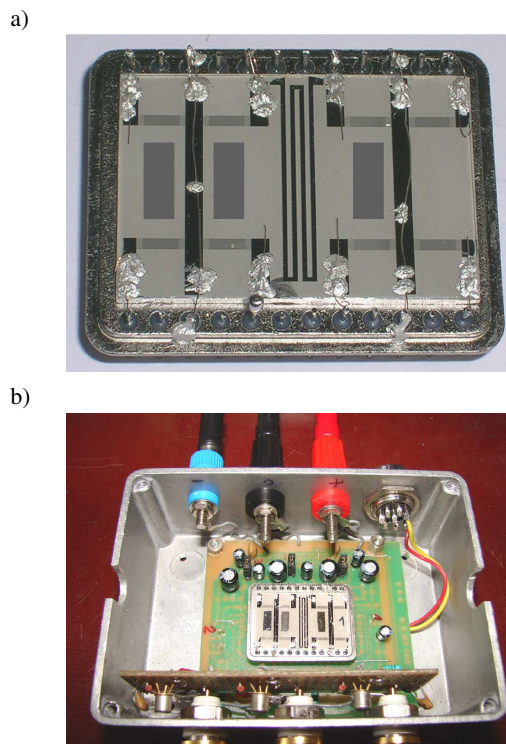
Fig. 10. The system of 4 acoustic lines on the LiNbO_3 substrate with 3 sensors layers and a reference line
