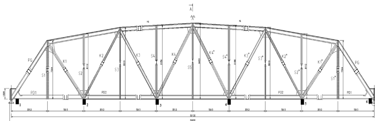
Fig. 14. Examed bridge span with sensors spaced on the bridge stringer (sensors 1, 2, 3, 4, 5, 6)
