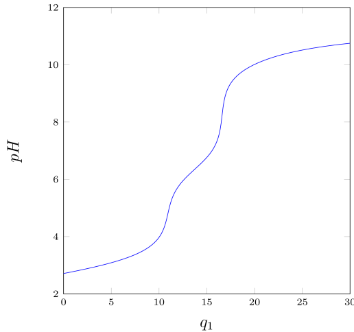
Figure 4. Static characteristic of the neutralization reactor
