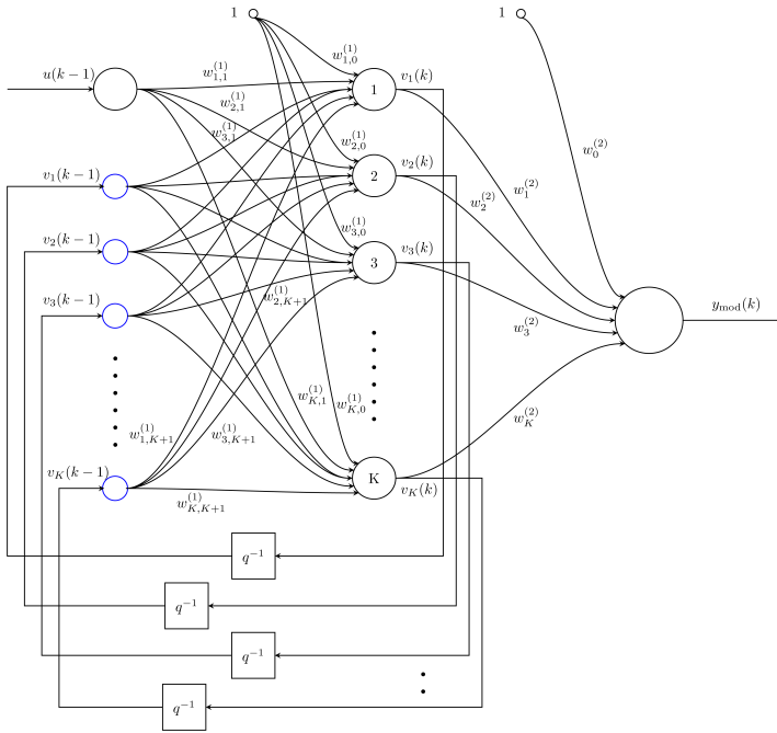
Figure 1. Structure of classical Elman neural network
