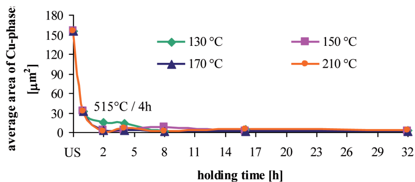
Fig. 7. Changes in average area of Cu-rich phases, (US – untreated state)
