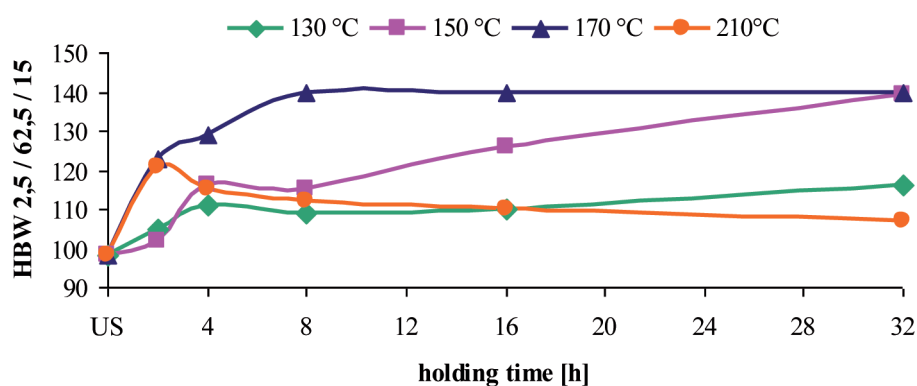
Fig. 8. Influence of heat treatment on hardness, (US – untreated state)
