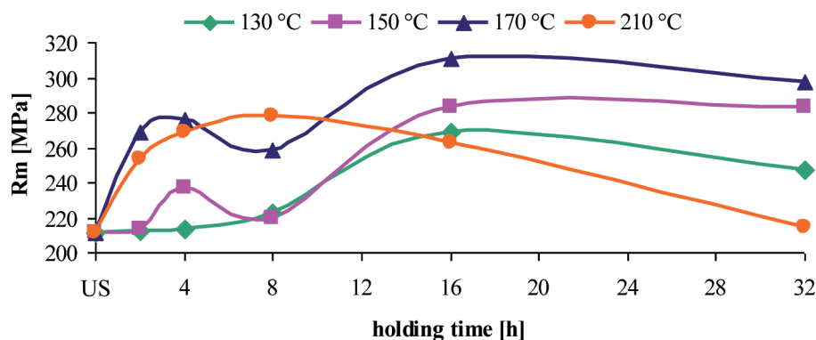
Fig. 9. Influence of heat treatment on strength tensile, (US – untreated state)
