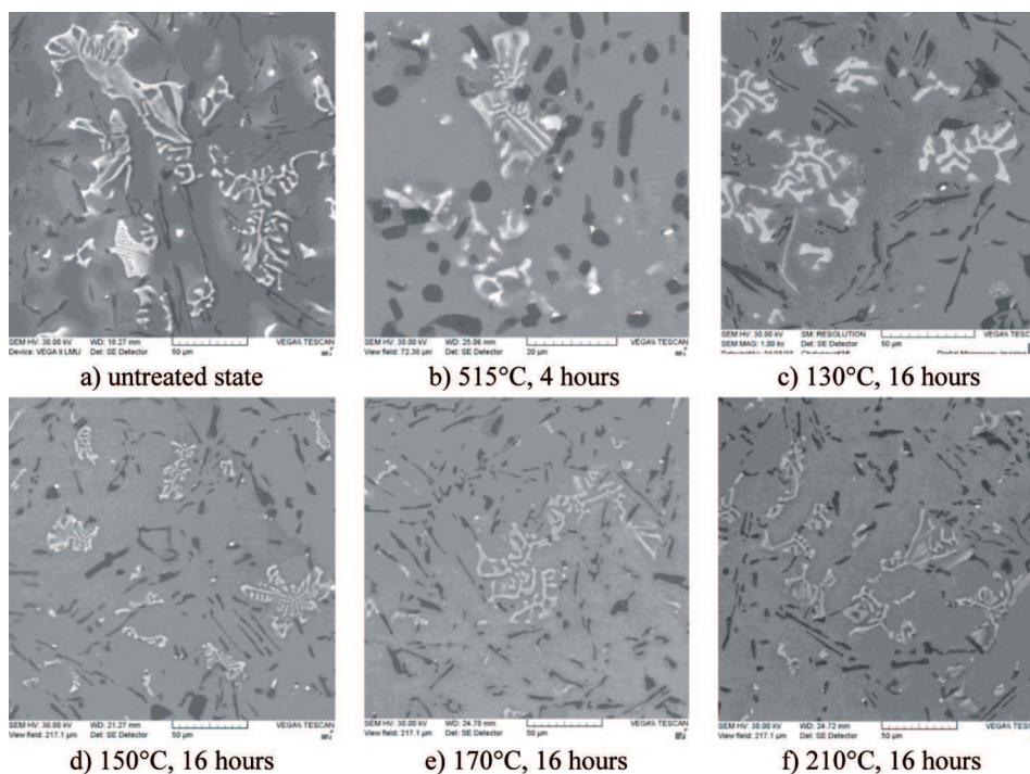
Fig. 3. Changes in morphology of Al_{15}(FeMn)_3Si_2 phases during age-hardening, etch. 0.5% HF, SEM
