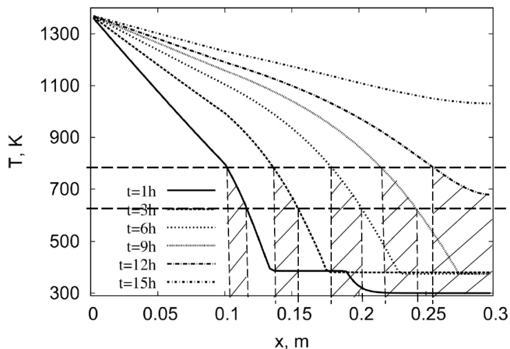
Fig. 9. Predicted temperature distribution within the coke oven (1/2 of the coke oven chamber) with the plastic layer zone marked (hatched areas)
