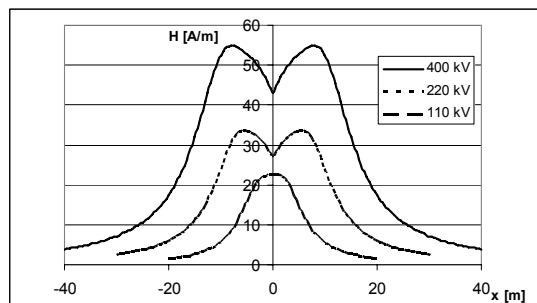
Fig. 4. Magnetic field intensity near 400 kV, 220 kV and 110 kV lines
